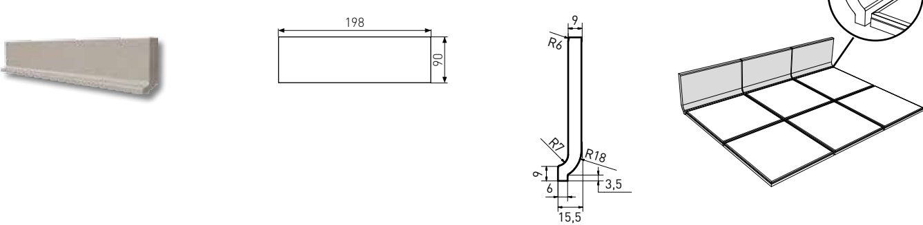
sokl s požlábkem | cove skirting | TSPEM... | 198×90×9 mm
