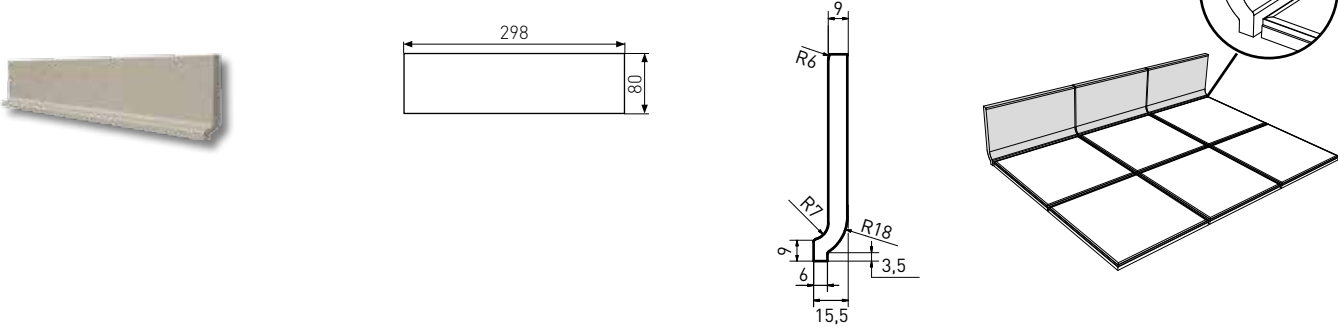
sokl s požlábkem | cove skirting | TSPJB... | 298×80×9 mm
