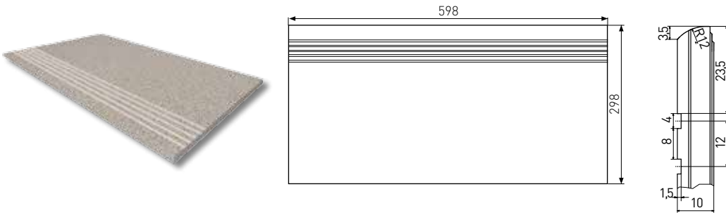
schodovka | step tile | TCPSA... | 298×598×10 mm
